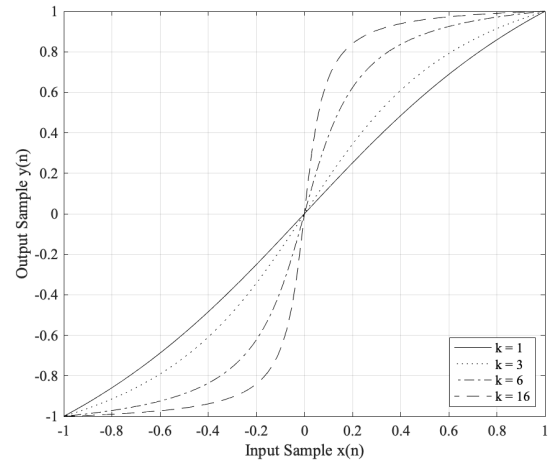
Figure 6. Input/output relationship of sigmoid waveshapers set to a range of parameter values.
