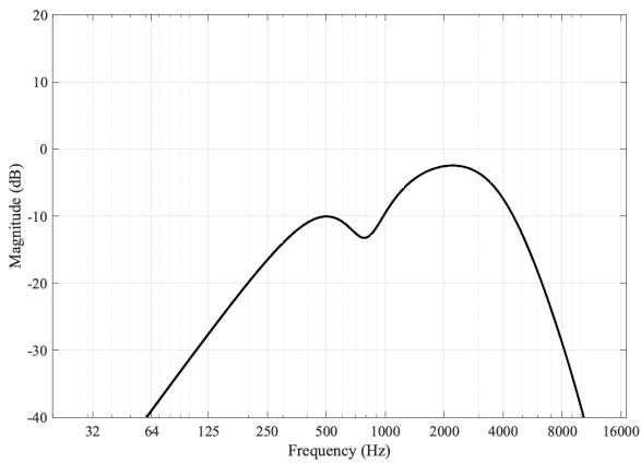
Figure 8. Magnitude response of the tuned post-filter for the Mercury model.
